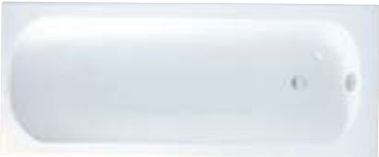
160x70cm standard bath, OTH White £271 – 50810001000 H: 380mm W: 1600mm P: 700mm
