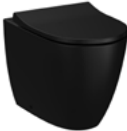
Back-to-wall WC pan, Rim-ex, 54cm Matt White £470 – 7985B001-0075 Matt Taupe £470 – 7985B020-0075 Matt Black £470 – 7985B083-0075 Black £470 – 7985B070-0075 H: 400mm W: 365mm P: 540mm
