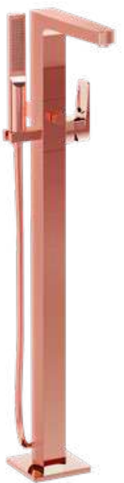
Floor-mounted bath mixer with hand shower, square • Soft Copper £1,409 - A4276029 H: 910mm P: 225mm
