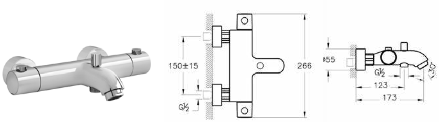
Aquaheat thermostatic bath/shower mixer P: 173mm
