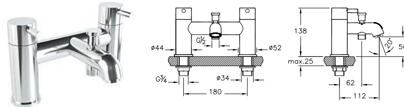
Minimax S deck-mounted bath/shower mixer with hand shower, 2TH H: 138mm P: 112mm
