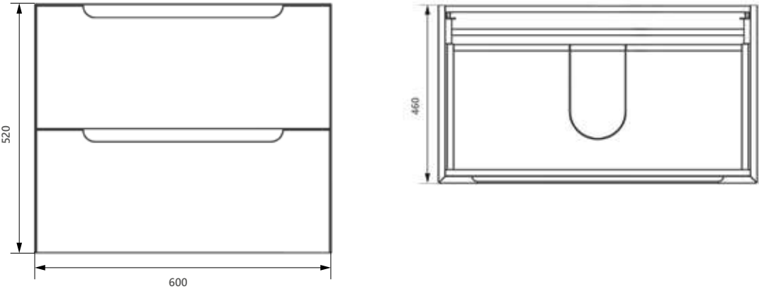
AT.620.800 Atoll 800mm wall hung unit
