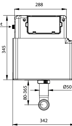
Concealed cistern for WC furniture unit
