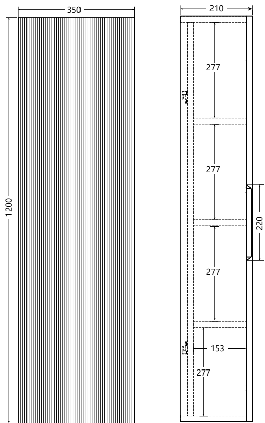
PA.650.1200 Palladium 1200mm 1 door wall hung unit
