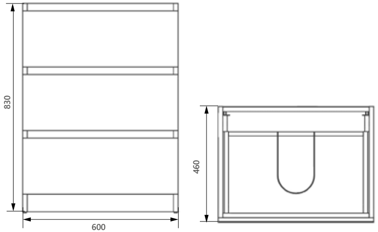
OP.630.600 Opa 600mm floor standing unit
