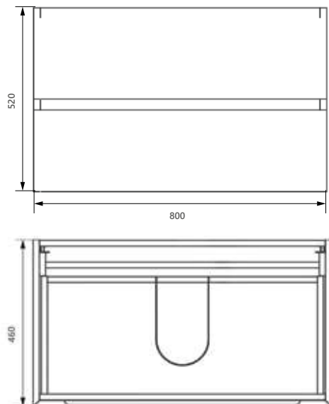
OP.620.800 Opa 800mm wall hung unit
