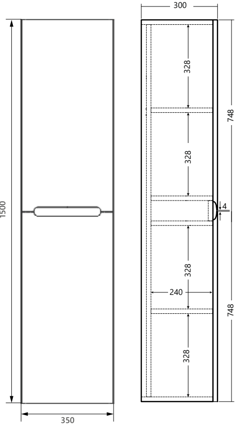
AT.650.1500 Atoll 1500mm wall hung cabinet
