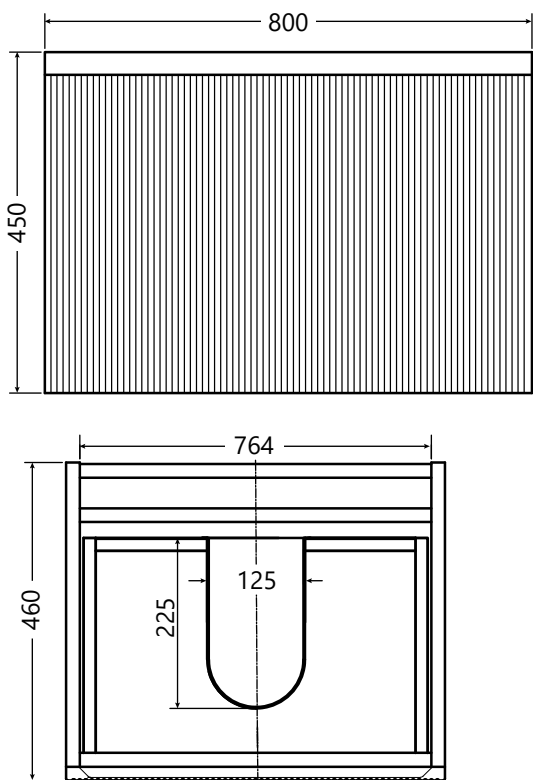
PA.611.800 Palladium 800mm wall hung unit with 1 outer drawer and 1 internal drawer
