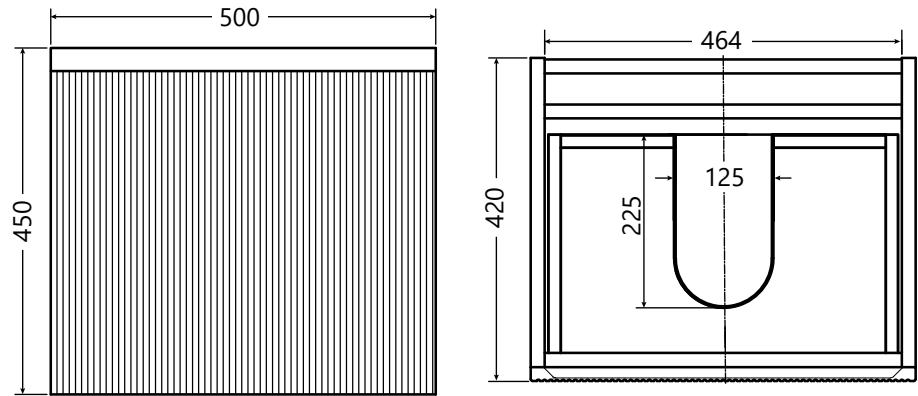
PA.611.500 Palladium 500mm wall hung unit with 1 outer drawer and 1 internal drawer
