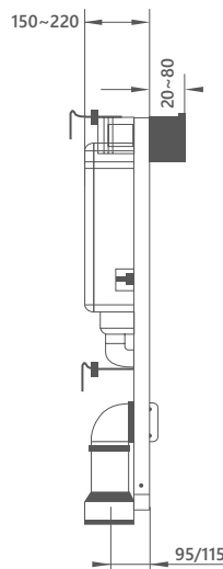
Flush plate mounted on front
