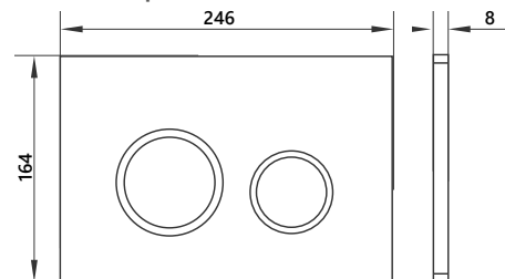
Halo flush plate for use with CI.732
