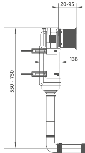
Flush plate mounted on front
