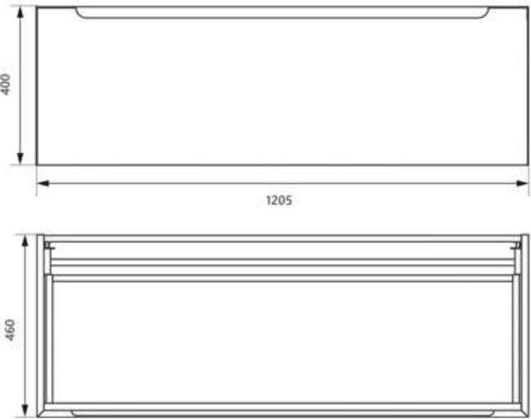
AT.610.1200 Atoll 1200mm wall hung unit
