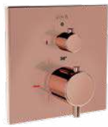
Built-in thermostatic bath mixer, 2-way, square Copper £224 – A4266826 Chrome £190 – A42668 Brushed Nickel £280 – A4266834 Gold £280 – A4266823 Matt Black £280 – A4266836 H: 170mm P: 60mm
