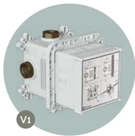
V-Box concealed shower valve £98 – A42263 H: 146mm P: 77-142mm
