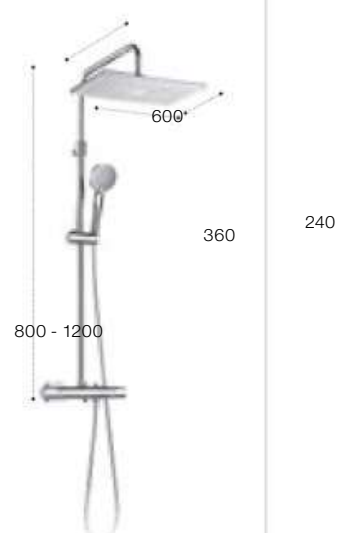
Wall-mounted shower column
