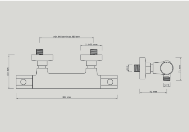
A47183 Essential thermostatic shower mixer £110* Recommended min pressure: 0.3 bar
