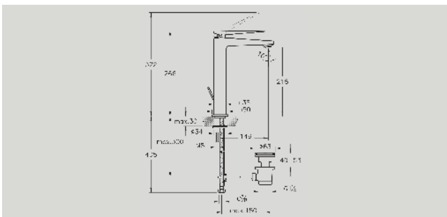
A42611 Tall basin mixer with pop-up waste £415 Recommended min pressure: 0.3 bar
