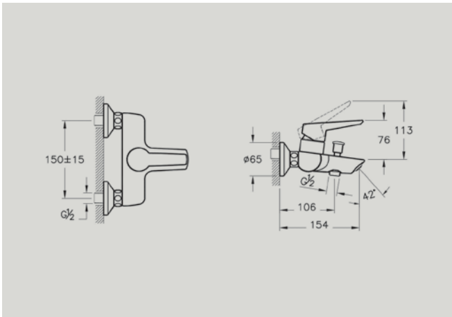
A42444 Wall-mounted bath/shower mixer £107* Recommended min pressure: 0.5 bar
