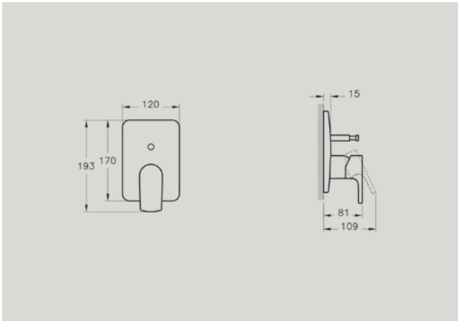
A42294 Built-in bath mixer, exposed part for A41949 £76* Recommended min pressure: 0.5 bar
