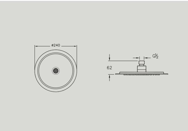
A45640 Lite showerhead £106*
