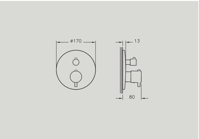
A42271 Built-in thermostatic bath/shower mixer, 2-way, exposed part for A42262 £163* Recommended min pressure: 1.0 bar
