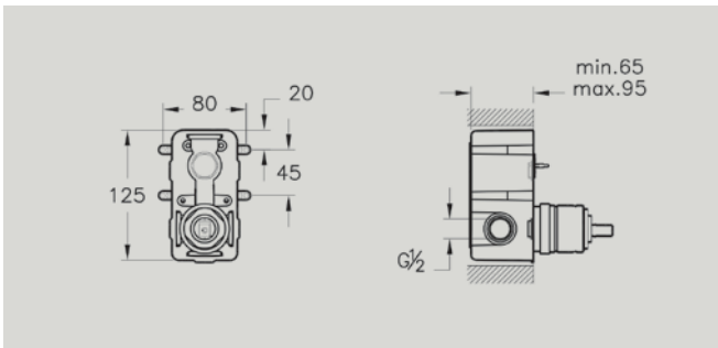
A41949 Minibox, 2-way, concealed part for A42251, A42286, A42294, A42446 £78* Recommended min pressure: 1.0 bar
