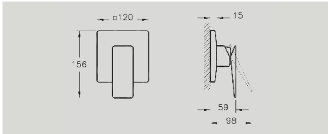
A42396 Built-in shower mixer, exposed part for A42213 £178* Recommended min pressure: 1.0 bar
