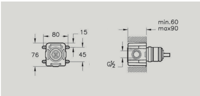
A42213 Minibox, 1-way, concealed part for A42295, A42287, A42447 £73* Recommended min pressure: 1.0 bar
