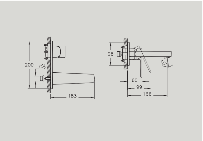
A42250 Built-in basin mixer, exposed part for A42230 £150* Recommended min pressure: 0.5 bar
