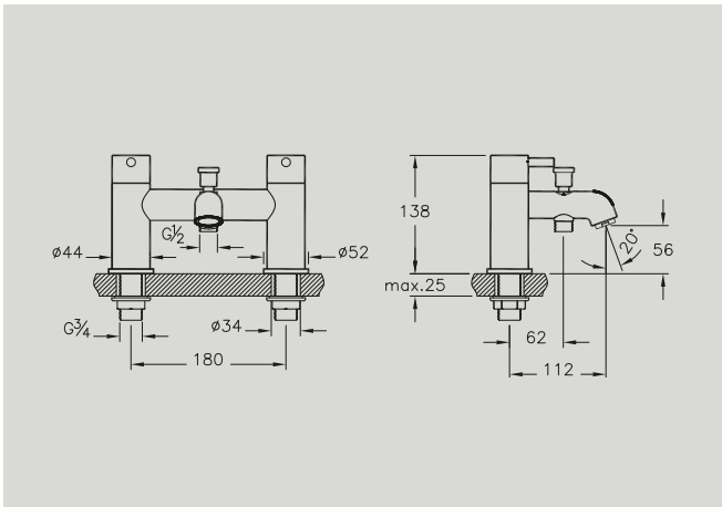
A42410 Deck-mounted bath/shower mixer (including handshower) £334* Recommended min pressure: 0.5 bar
