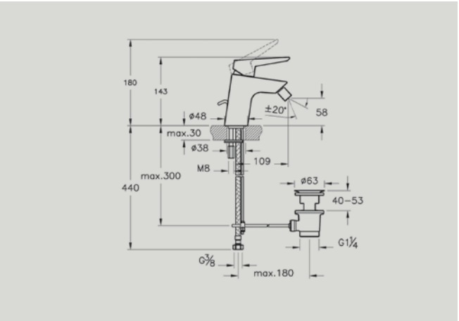
A42443 Bidet mixer with pop-up waste £96* Recommended min pressure: 0.3 bar
