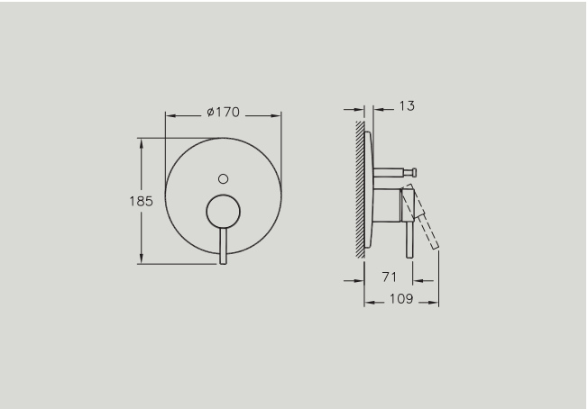
A42265 Built-in bath/shower mixer, 2-way, exposed part for A42262 £109* Recommended min pressure: 1.0 bar
