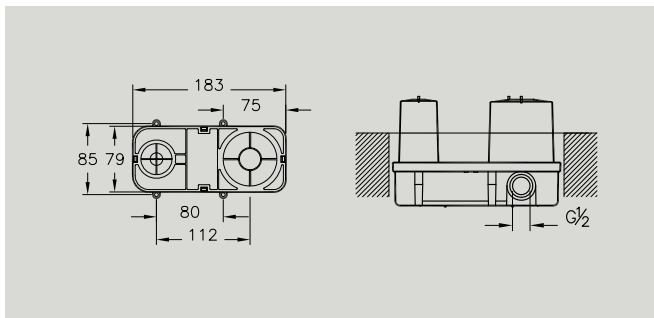
A42230 Built-in basin mixer, concealed part for A42394 £97 Recommended min pressure: 0.5 bar
