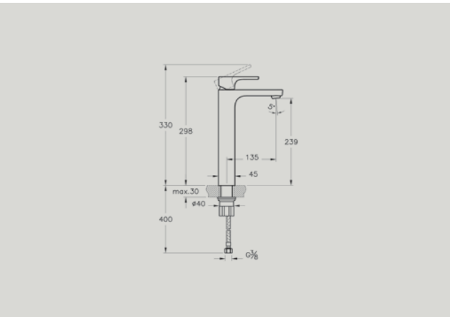
A42514 Tall basin mixer with top handle £171* Recommended min pressure: 0.5 bar
