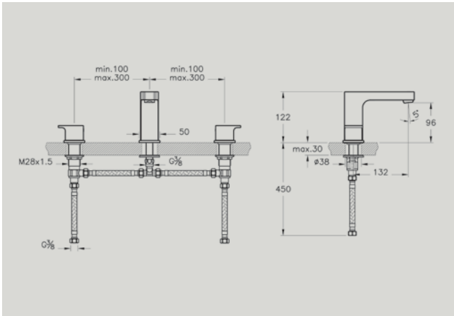
A42507 Basin mixer, 3TH £183* Recommended min pressure: 0.5 bar
