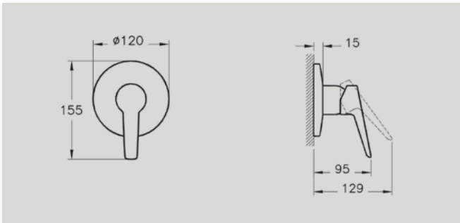
A42447 Solid S built-in shower mixer, exposed part for A42213 £68* Recommended min pressure: 1.0 bar
