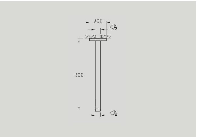
Long connection pipe, ceiling-mounted: NEW A45650 Chrome £68* A4565026 Copper £82* A4565034 Brushed nickel £102* A4565036 Matt black £102*
