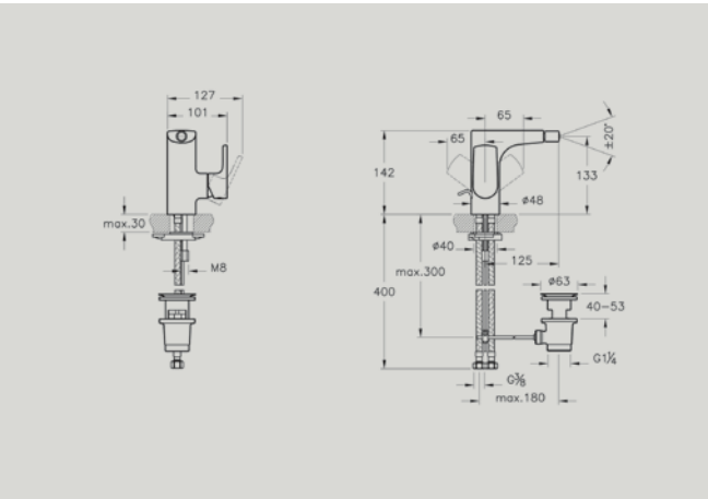
A42519 Bidet mixer with pop-up waste £190* Recommended min pressure: 0.5 bar
