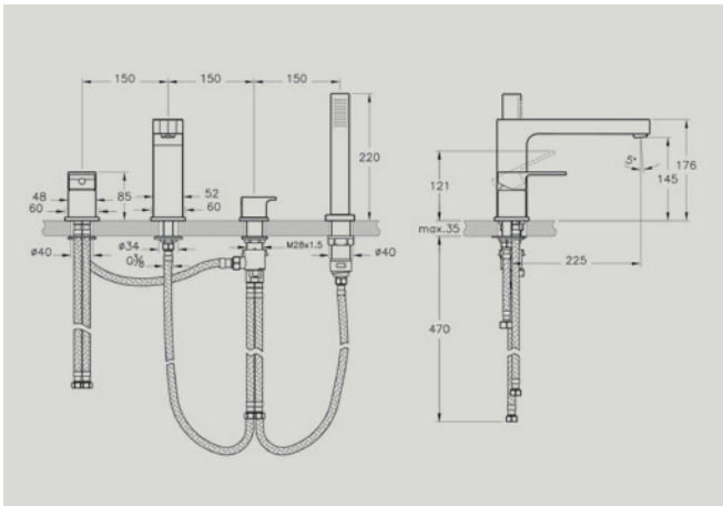
A42531 Deck-mounted bath mixer, 4TH (including handshower) £389* Recommended min pressure: 1.0 bar
