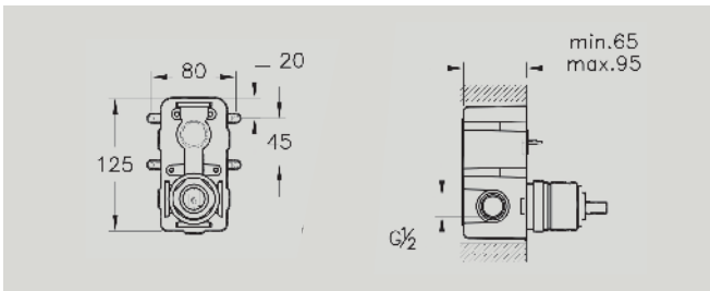
A41949 Minibox, 2-way, concealed part for A42395 £78* Recommended min pressure: 1.0 bar
