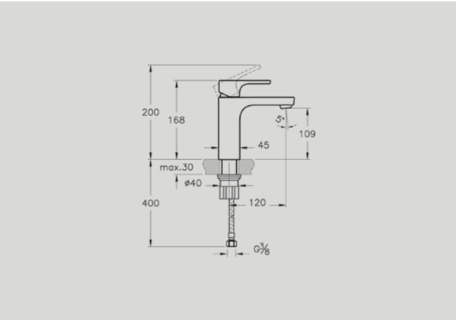
A42513 Basin mixer with top handle £127* Recommended min pressure: 0.5 bar
