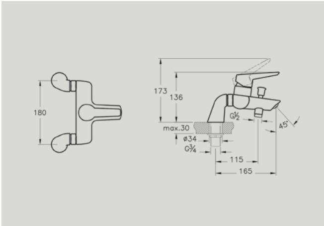
A42498 Deck-mounted bath/shower mixer, with handshower £199* Recommended min pressure: 0.5 bar
