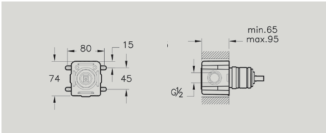
A42213 Minibox, 1-way, concealed part for A42396 £73* Recommended min pressure: 1.0 bar
