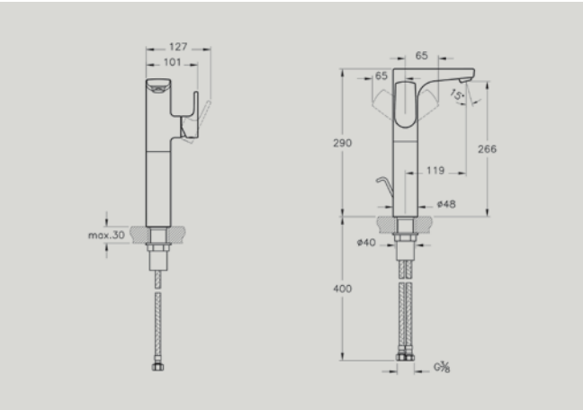
A42523 Tall basin mixer with side handle £197* Recommended min pressure: 0.5 bar
