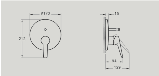
A42446 Solid S built-in bath/shower mixer, exposed part for A41949 £76* Recommended min pressure: 1.0 bar
