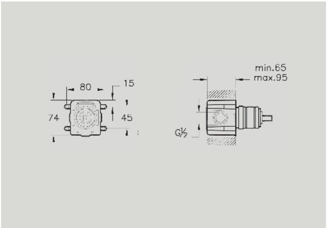
A42213 Minibox, 1-way, concealed part for A42295 £73* Recommended min pressure: 1.0 bar
