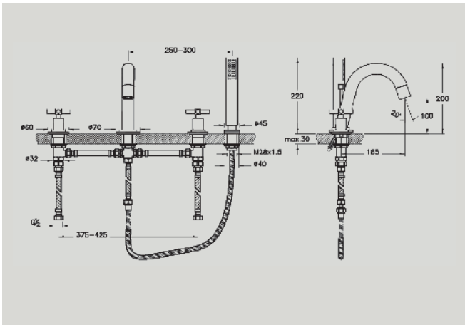
Deck-mounted bath mixer, 4TH: NEW A40935 Chrome £533* A4093523 Gold £639* Recommended min pressure: 1.0 bar
