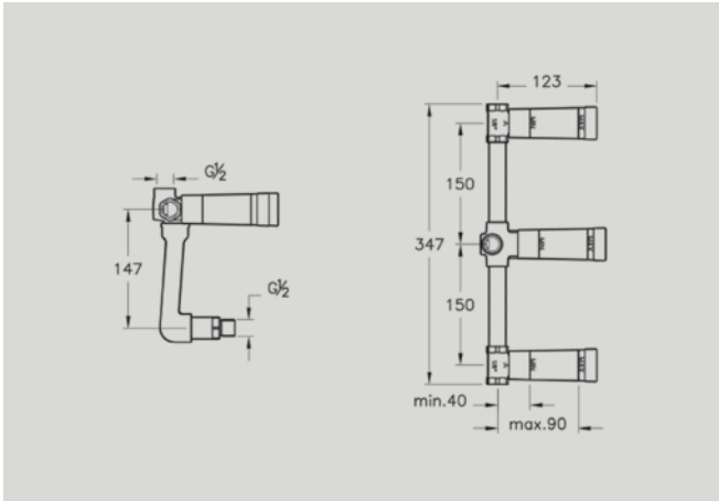
A40834 Built-in bath/shower mixer, concealed part for A40831 and A40832 NEW £80* Recommended min pressure: 1.0 bar
