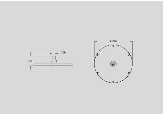
Vichy XL showerhead: NEW A45638 Chrome £160* A4563826 Copper £191* A4563834 Brushed nickel £239* A4563836 Matt black £239* Recommended min pressure: 1.0 bar
