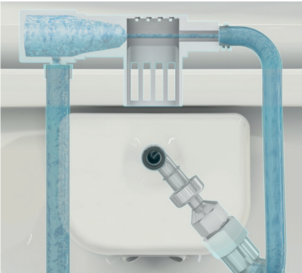
Close-up of the integrated air breaker
