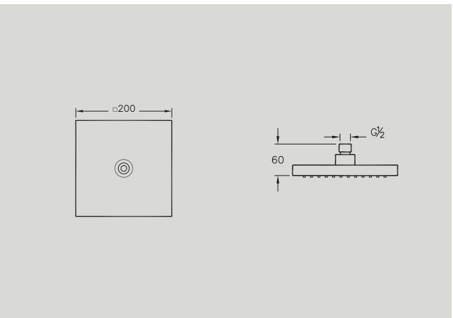
A45707 Rain Q showerhead £53*
