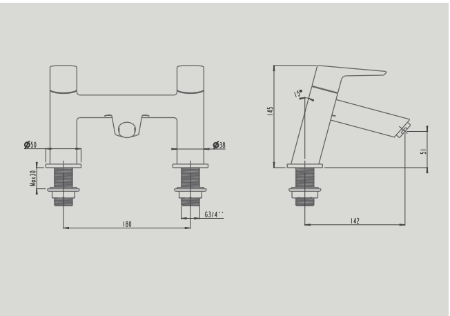
A42416 Deck-mounted bath mixer, 2TH £249* Recommended min pressure: 0.5 bar
