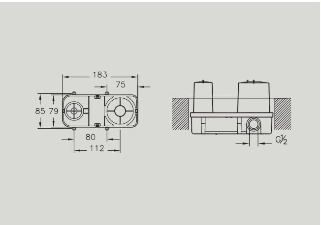
A42230 Built-in basin mixer, concealed part for A42250 £97* Recommended min pressure: 0.5 bar
