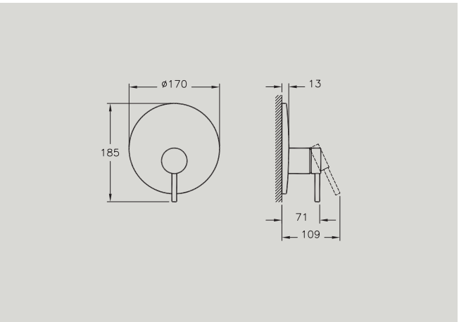
A42268 Built-in shower mixer, 1-way, exposed part for A42262 £98* Recommended min pressure: 1.0 bar
