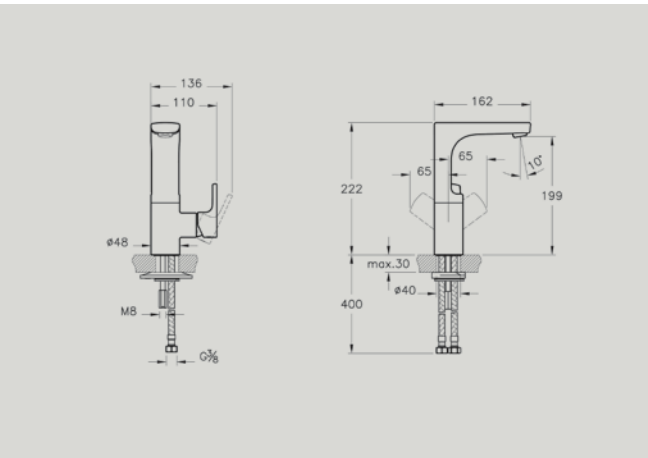
A42524 Basin mixer with side handle and swivel spout £178* Recommended min pressure: 0.5 bar
