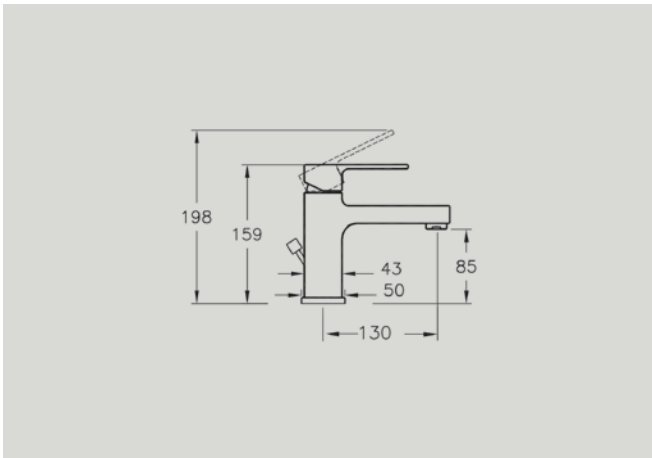
A40776 Basin mixer with pop-up waste £197* Recommended min pressure: 0.3 bar
