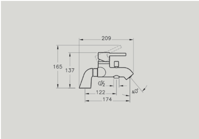
A42112 Deck-mounted bath/shower mixer (including handshower) £296* Recommended min pressure: 1.0 bar
