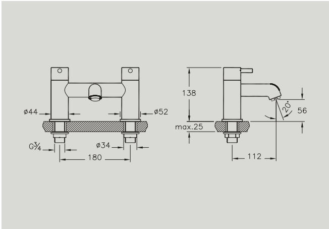
A42411 Deck-mounted bath filler £290* Recommended min pressure: 0.5 bar
