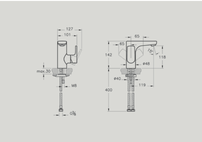
A42521 Basin mixer with side handle £146* Recommended min pressure: 0.5 bar
