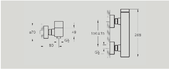
A42614 Shower mixer £440* Recommended min pressure: 0.5 bar
