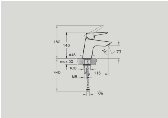
A42440 Basin mixer £75* Recommended min pressure: 0.3 bar
