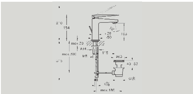
A42609 Basin mixer with pop-up waste £283 Recommended min pressure: 0.3 bar
