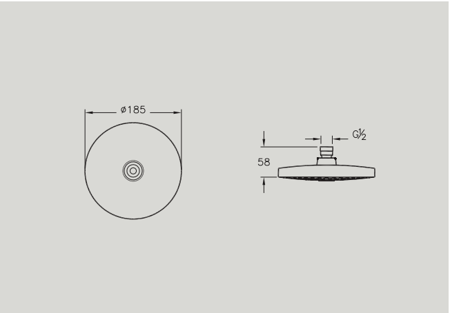
A45708 Rain L showerhead £54*
