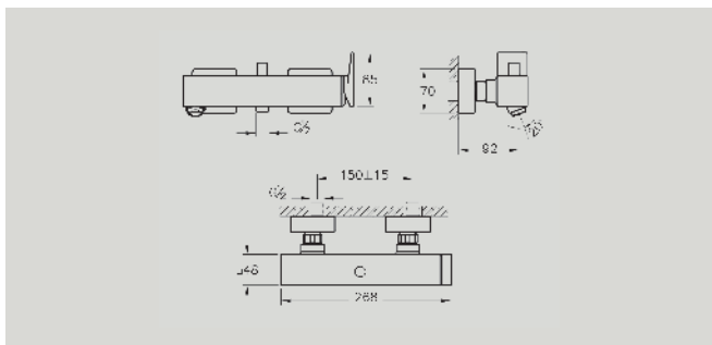
A42613 Bath/shower mixer £628 Recommended min pressure: 0.5 bar
