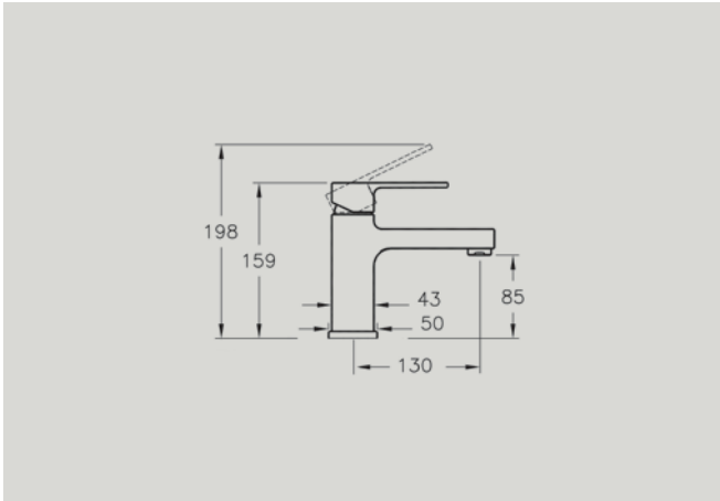
A40775 Basin mixer £160* Recommended min pressure: 0.3 bar
