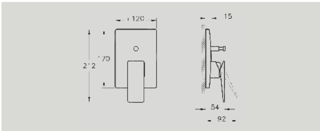
A42395 Built-in bath/shower mixer, exposed part for A41949 £183* Recommended min pressure: 1.0 bar
