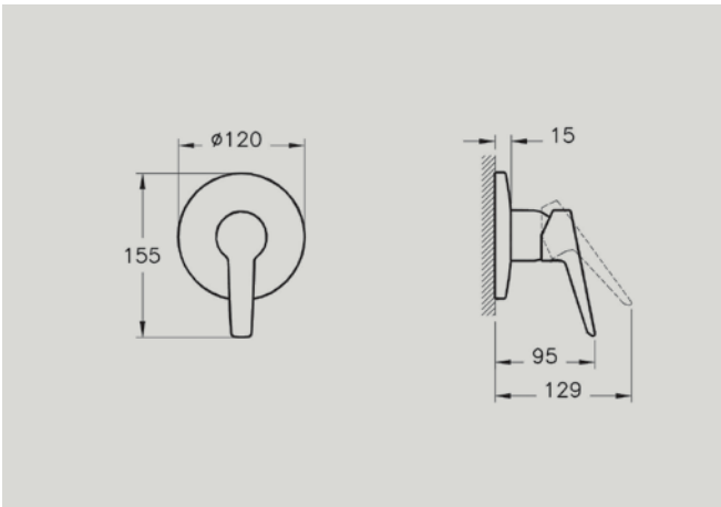
A42447 Built-in shower mixer, exposed part for A42213 £68* Recommended min pressure: 1.0 bar
