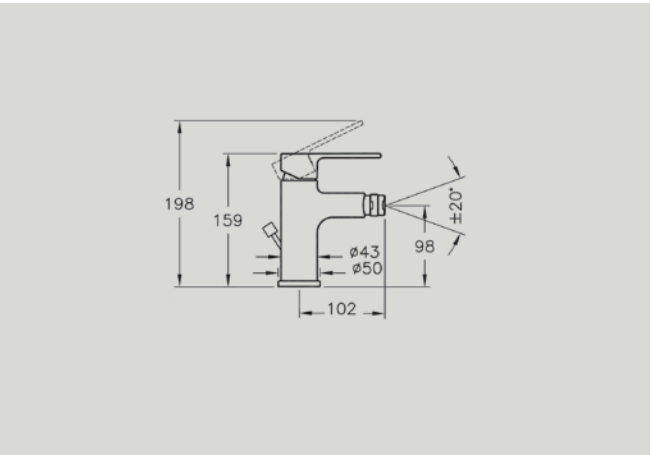
A40777 Bidet mixer with pop-up waste £223* Recommended min pressure: 0.3 bar
