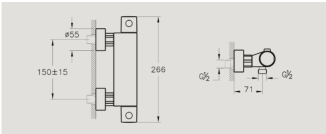
A47174 Aquaheat RS3 shower mixer NEW £180* Recommended min pressure: 1.5 bar
