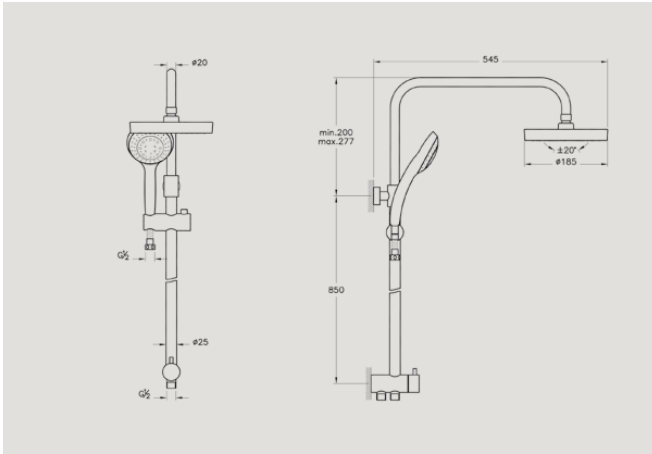
A45597 System rain shower column £403* Recommended min pressure: 1.0 bar
