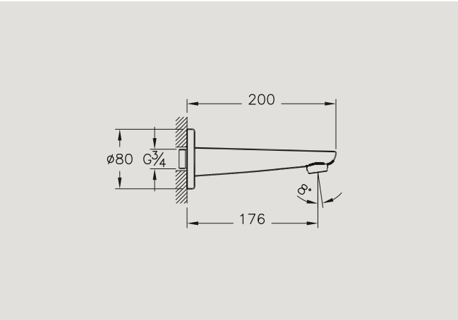
A40699 Bath spout £85*
