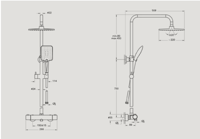
A49253 Aquaheat RH3 thermostatic shower system, square NEW £410* Recommended min pressure: 1.5 bar
