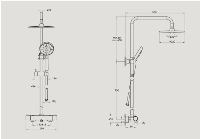
A49252 Aquaheat RH3 thermostatic shower system, round NEW £390* Recommended min pressure: 1.5 bar
