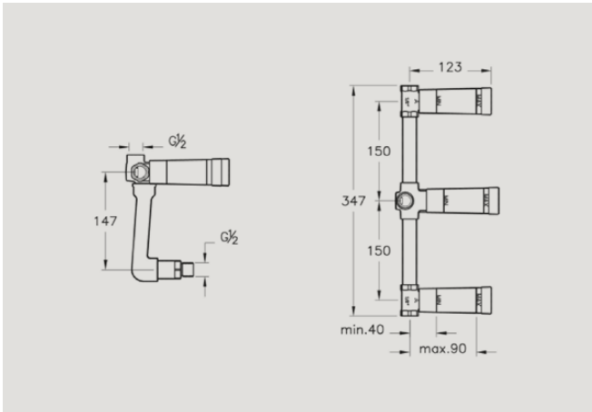
A40834 Built-in bath/shower mixer, concealed part for A40831 NEW £80* Recommended min pressure: 1.0 bar
