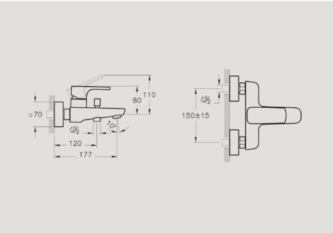
A42516 Wall-mounted bath mixer £165* Recommended min pressure: 1.0 bar
