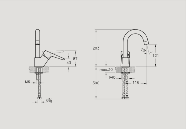
A42442 Basin mixer with swivel spout £100 Recommended min pressure: 0.3 bar
