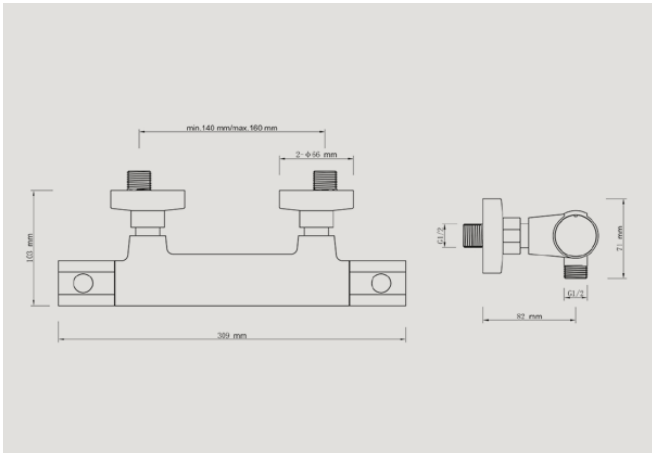
A47183 Essential thermostatic shower mixer NEW £110* Recommended min pressure: 0.3 bar
