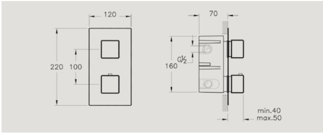
A47163 Aquaheat thermostatic mixer, 2-way (includes concealed part) £275* Recommended min pressure: 1.0 bar
