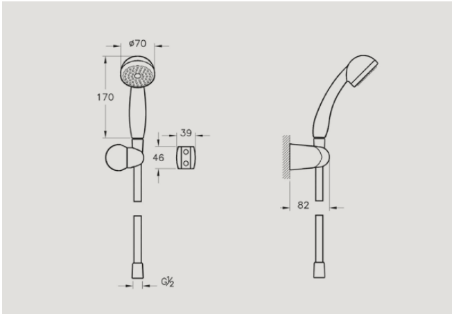
A45675 Solo C handshower without slide rail £48* Recommended min pressure: 1.0 bar
