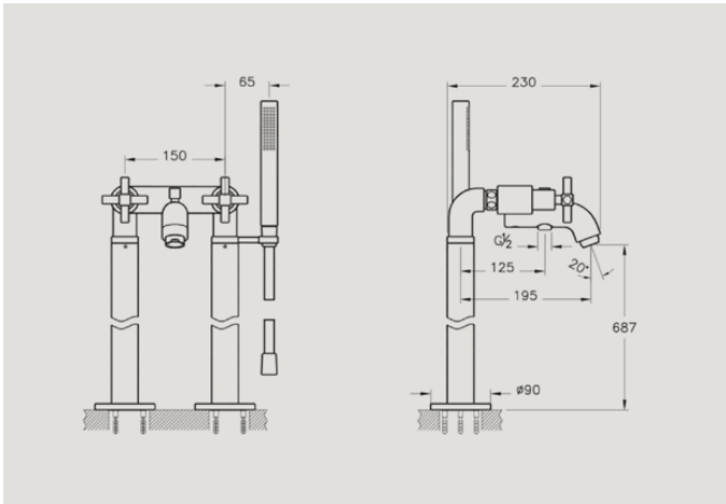
Floor-mounted bath mixer (including handshower): NEW A42398 Chrome £746* A4239823 Gold £895* Recommended min pressure: 1.0 bar
