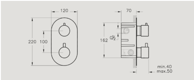
A47025 Aquaheat thermostatic mixer, 2-way (includes concealed part) £250* Recommended min pressure: 1.0 bar
