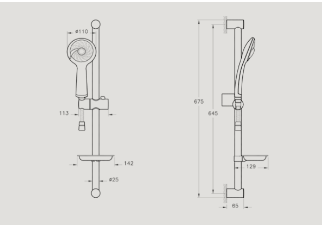
A45680 Samba handshower with slide rail, 3 functions £89* Recommended min pressure: 1.0 bar
