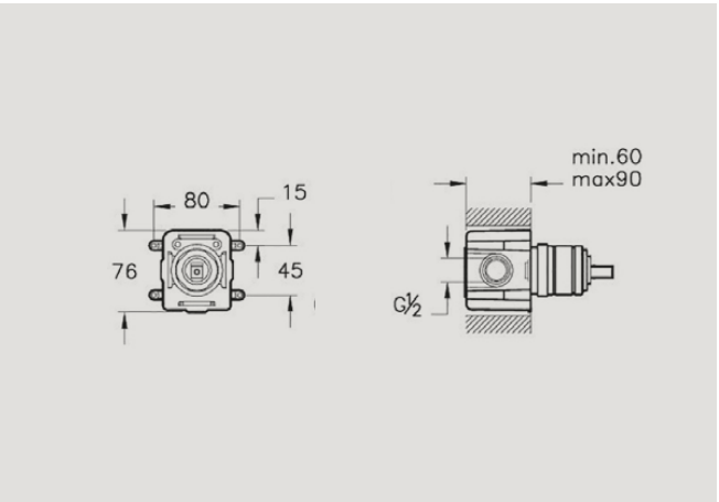
A42213 Minibox, 1-way, concealed part for A42447 £73* Recommended min pressure: 1.0 bar
