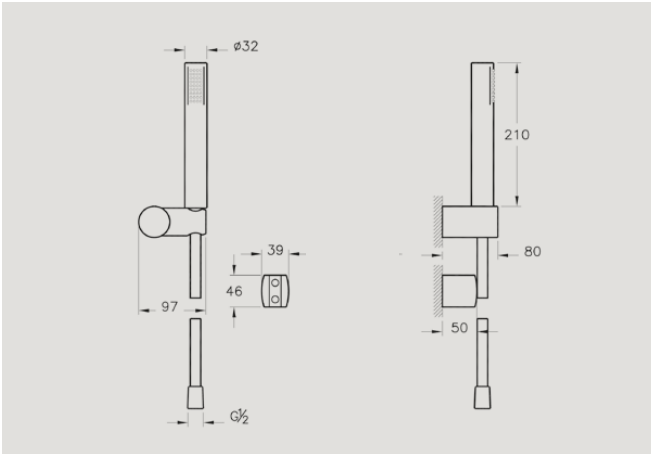
A45683 Sense handshower without slide rail £66* Recommended min pressure: 1.0 bar
