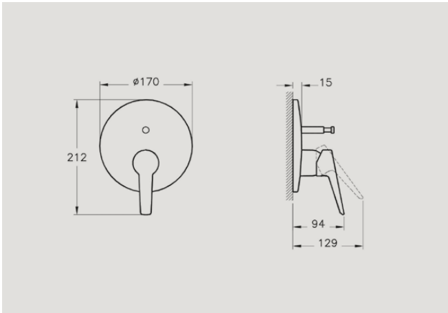
A42446 Built-in bath/shower mixer, exposed part for A41949 £76* Recommended min pressure: 1.0 bar
