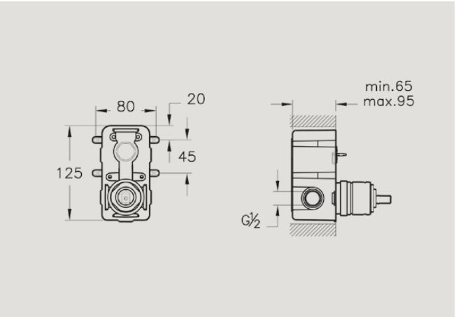
A41949 Minibox, 2-way, concealed part for A42446 £78* Recommended min pressure: 1.0 bar
