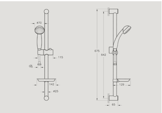
A45676 Solo C handshower with slide rail £80* Recommended min pressure: 1.0 bar
