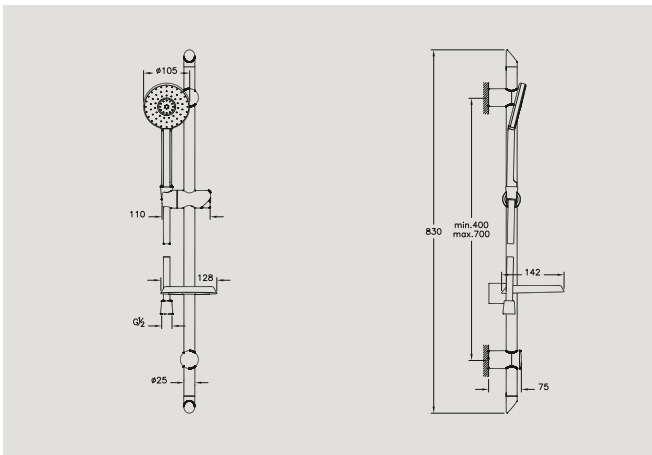
A45538 Style X handshower with slide rail £122* Recommended min pressure: 1.0 bar
