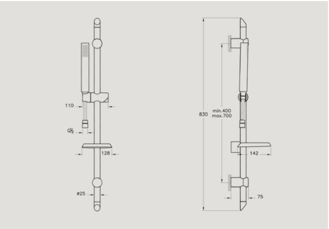
A45684 Sense handshower with slide rail £98* Recommended min pressure: 1.0 bar
