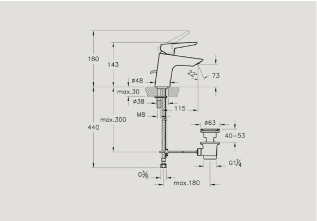
A42441 Basin mixer with pop-up waste £83 Recommended min pressure: 0.3 bar
