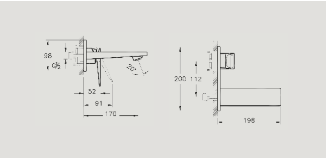
A42394 Built-in basin mixer, exposed part for A42230 £321* Recommended min pressure: 0.5 bar
