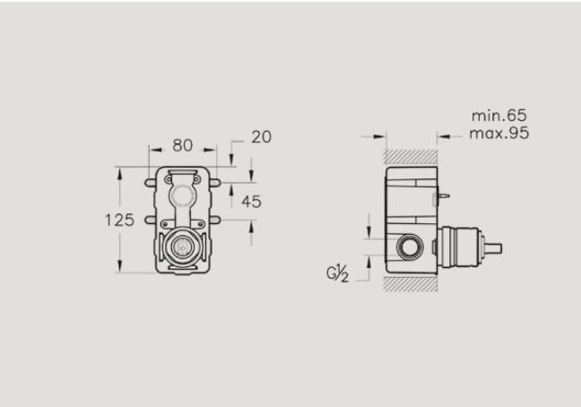
A41949 Minibox, 2-way, concealed part for A42294 £78* Recommended min pressure: 1.0 bar
