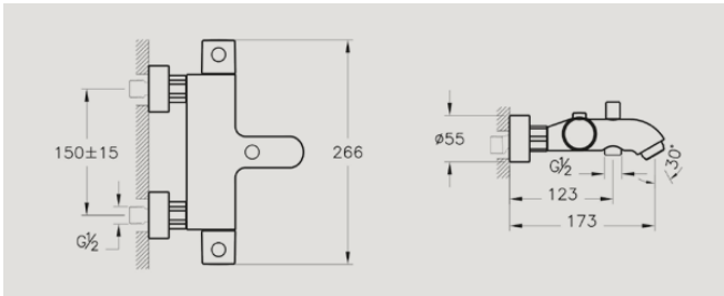
A47172 Aquaheat RS3 bath/shower mixer NEW £210* Recommended min pressure: 1.5 bar
