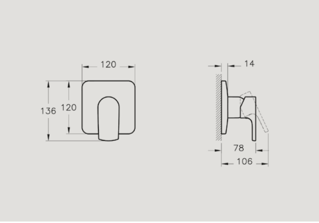
A42295 Built-in shower mixer, exposed part for A42213 £70* Recommended min pressure: 1.0 bar
