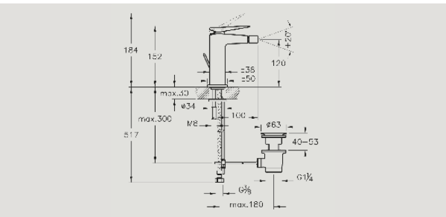
A42612 Bidet mixer £321* Recommended min pressure: 0.3 bar
