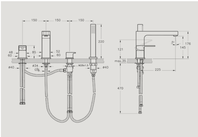
A42531 Bath mixer, 4TH (including handshower) £389* Recommended min pressure: 1.0 bar
