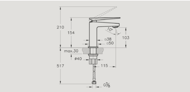
A42608 Basin mixer £251* Recommended min pressure: 0.3 bar
