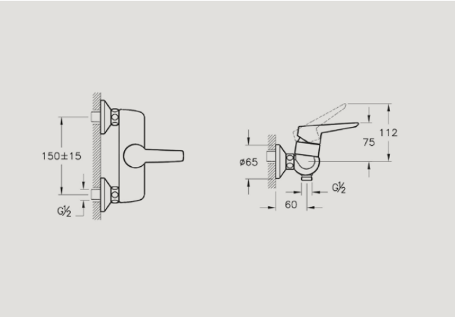
A42445 Shower mixer £87* Recommended min pressure: 0.5 bar
