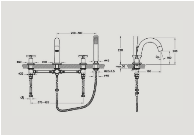
Bath mixer, 4TH: NEW A40935 Chrome £533* A4093523 Gold £639* Recommended min pressure: 1.0 bar
