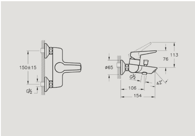
A42444 Bath/shower mixer £107* Recommended min pressure: 0.5 bar
