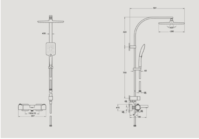
A49256 Aquaheat SS3 thermostatic bath/shower system, square NEW £658* Recommended min pressure: 1.5 bar
