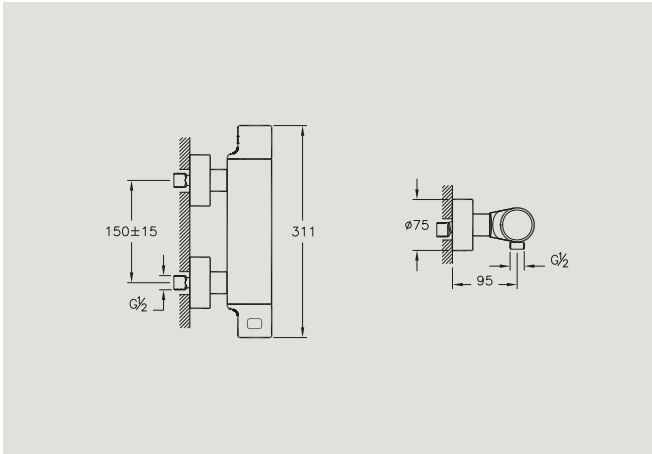
A47098 X-Line thermostatic shower mixer £120* Recommended min pressure: 1.0 bar
