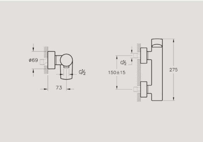
A42526 Shower mixer £149* Recommended min pressure: 1.0 bar
