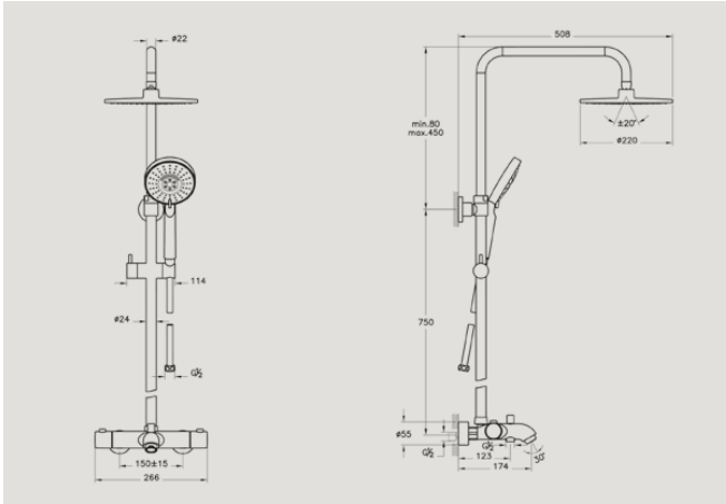
A49254 Aquaheat RH3 thermostatic bath/shower system, round NEW £488* Recommended min pressure: 1.5 bar
