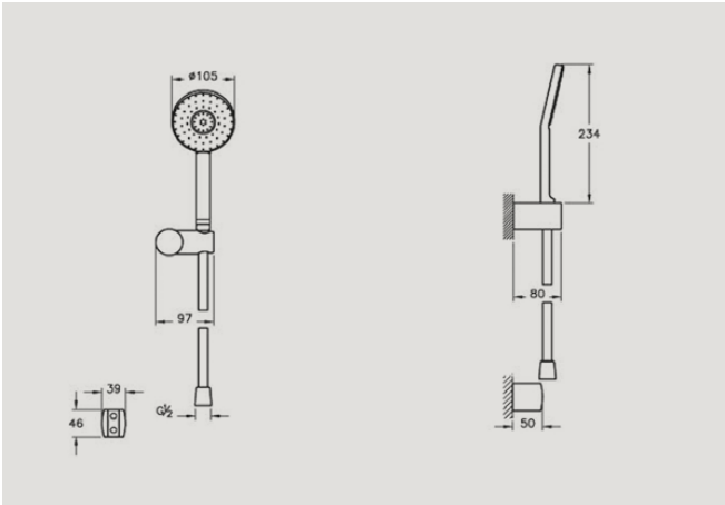
A45539 Style X handshower without slide rail £89* Recommended min pressure: 1.0 bar
