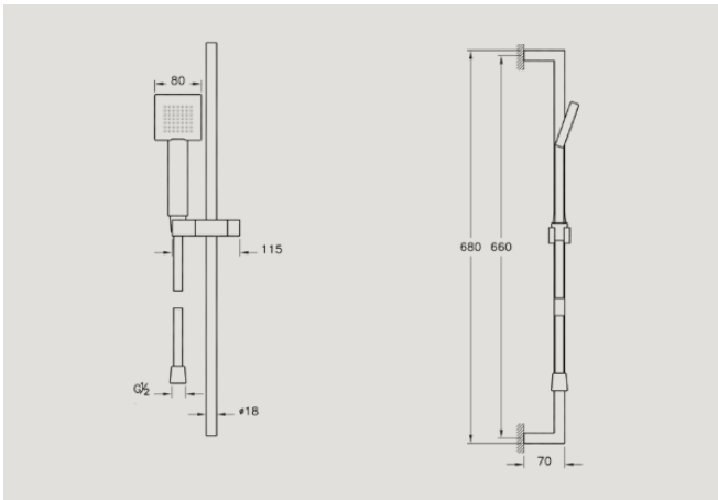
A45610 Q-Line handshower with slide rail £215* Recommended min pressure: 1.0 bar
