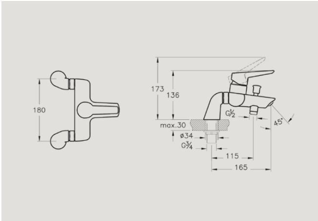
A42498 Bath/shower mixer, with handshower £199* Recommended min pressure: 0.5 bar
