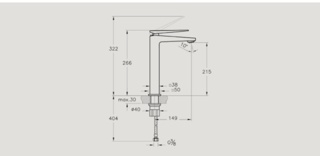
A42610 Tall basin mixer £374* Recommended min pressure: 0.3 bar
